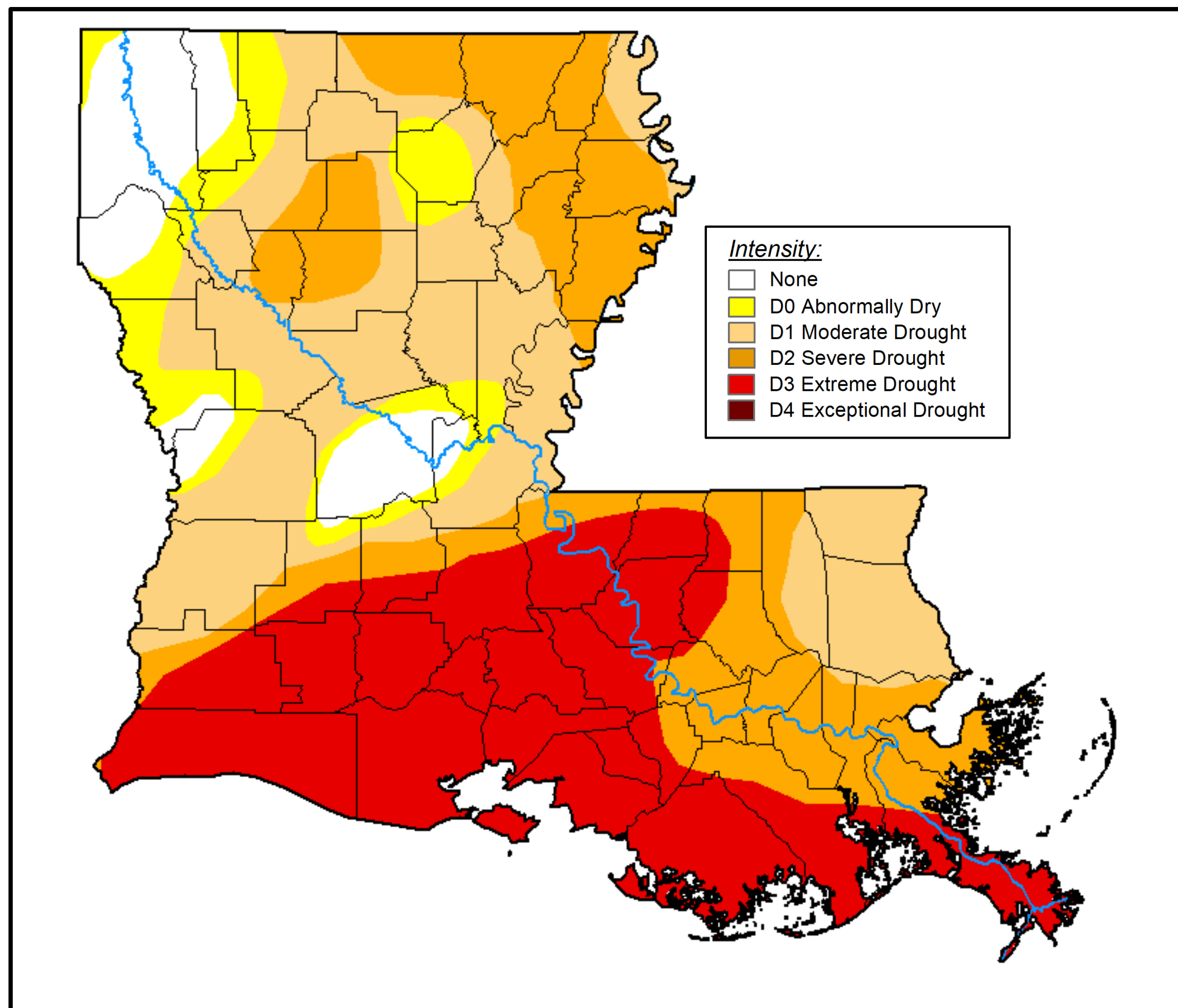
Louisiana Drought Monitor: Released 4/5/22
