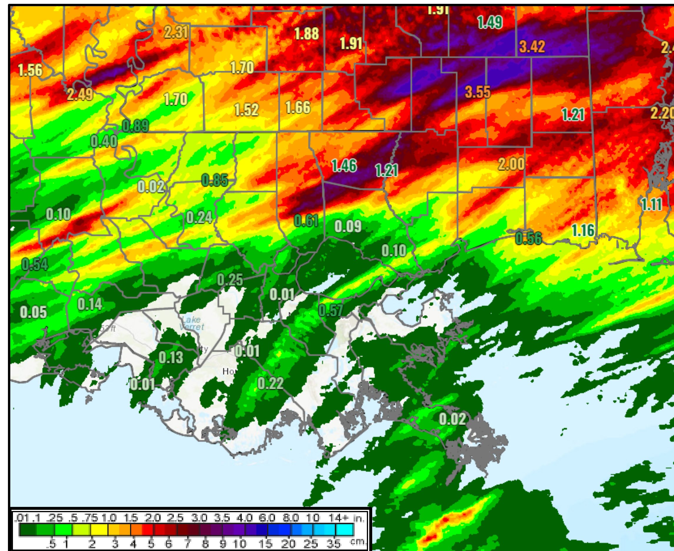
3 Day Rainfall Totals: 8AM Mon 4/4 thru 8AM Thu 4/7
